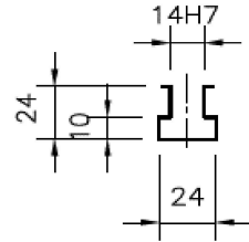
T槽尺寸 Width of T-Slot
