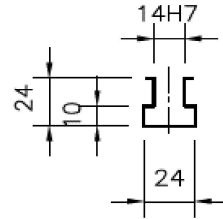
T槽尺寸 Width of T-Slot
