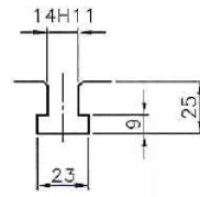
T槽尺寸 Width of T-Slot
